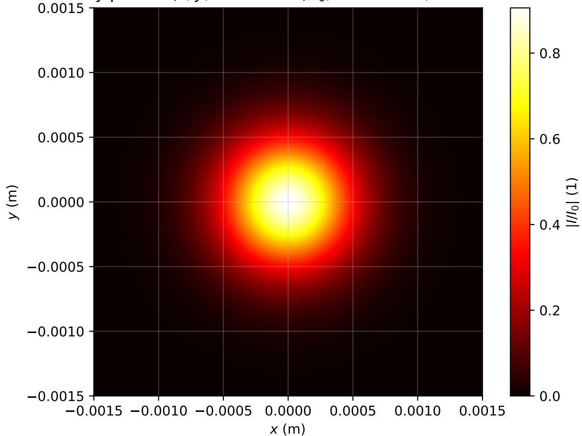
Intensity profile I(x, y, z = 1.115m)/I_0 , \text{Pin}=0.3\text{Pcr} , artificial time
